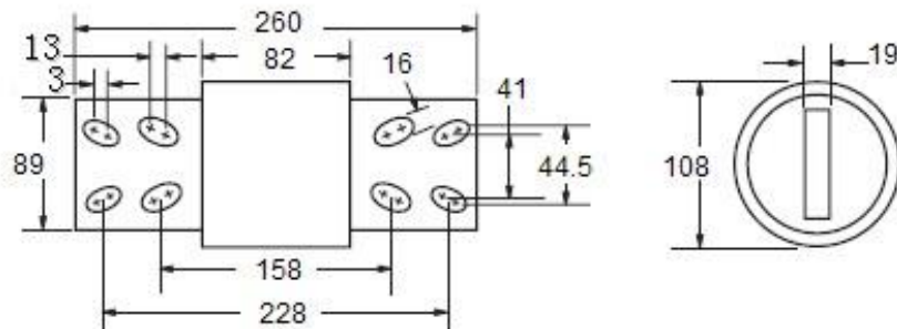
Figure 2: 1400 – 1600 Amp Range
