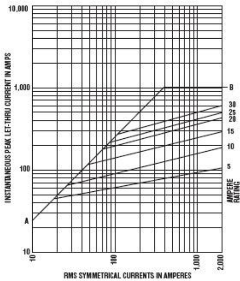
5 – 30 Amps, 700 Volts
