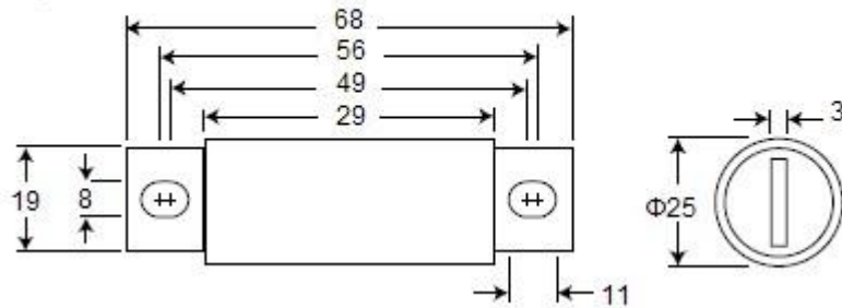
Fig. 2: 500-1000A
