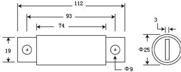
Fig. 2: 70-100A
