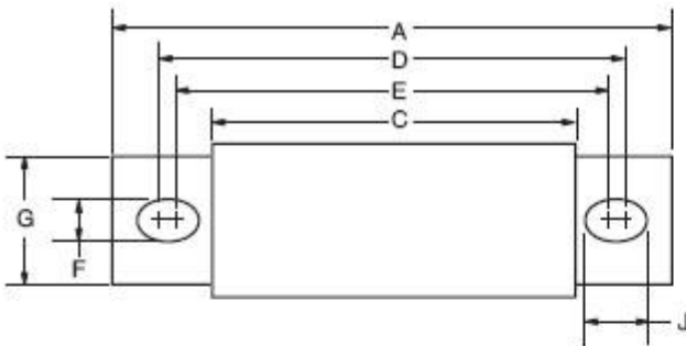
Figure 1: 35 – 100 & 125 – 800 Amp Range
