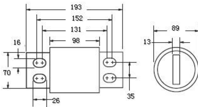
Figure 2: 900 – 1000 Amp Range
