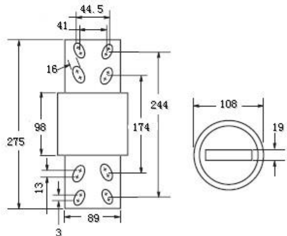
Figure 3: 1200 Amp Range
