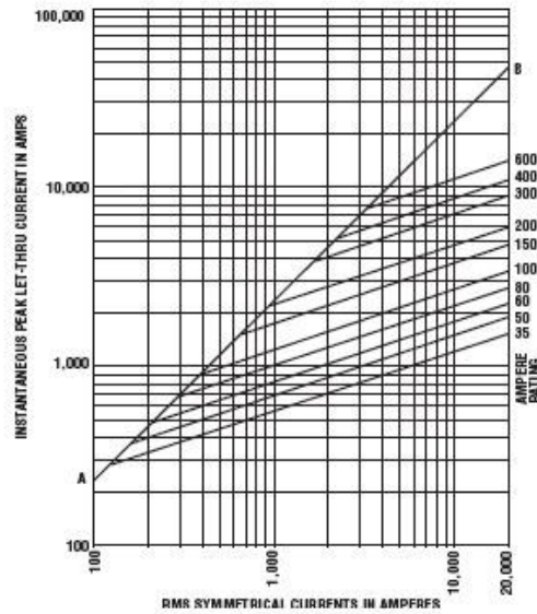
35 – 600 Amps, 700 Volts
