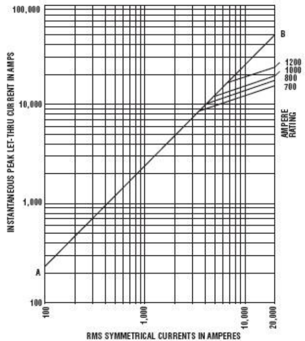
700 – 1200 Amps, 700 Volts
