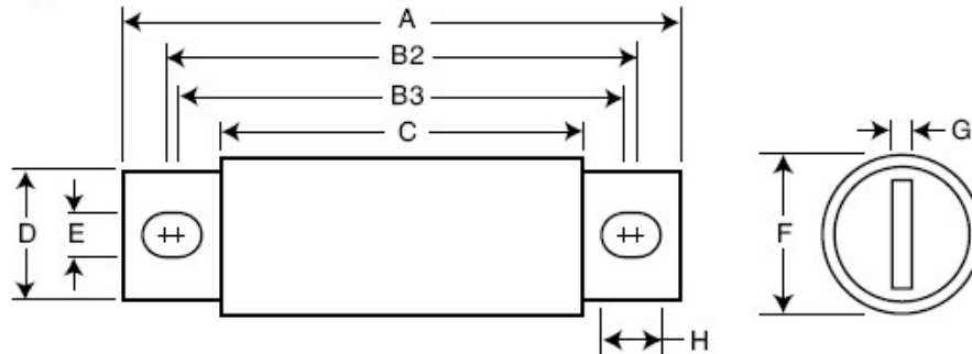
Fig. 2: 35-400A
