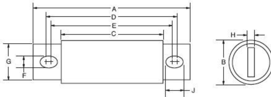
Figure 1: 35 – 1200 Amp Range
