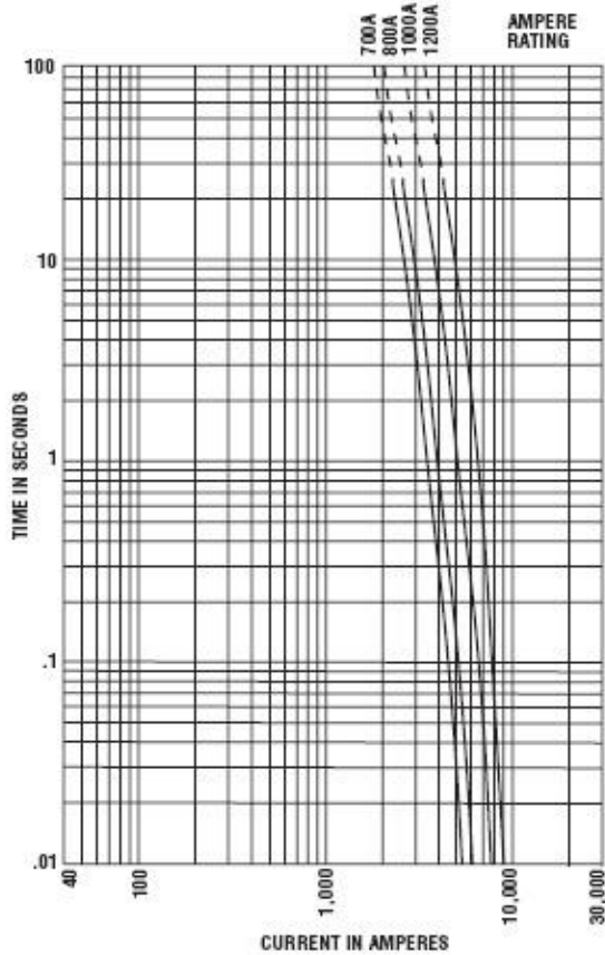
700 – 1200 Amps, 700 Volts
